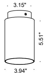
Fixture Dimensions
