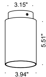
Fixture Dimensions
