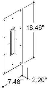
T131197 Frame for plaster 9.06 x 2.24 in Installation depth 2.20 in
