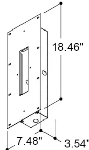
T131177 Frame + Box for plaster 16.97 x 4.49 in Installation depth 3.54 in
