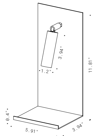
Fixture dimensions
