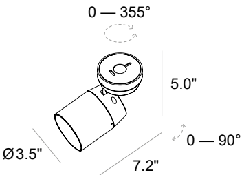
Fixture Dimensions
