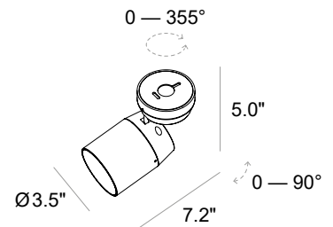
Fixture Dimensions
