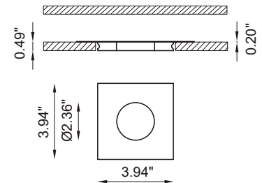
Fixture Dimensions:
