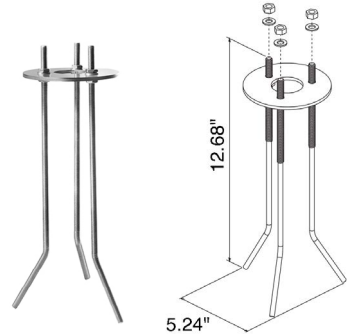
WULL10A0 Anchor Kit with Bolts
