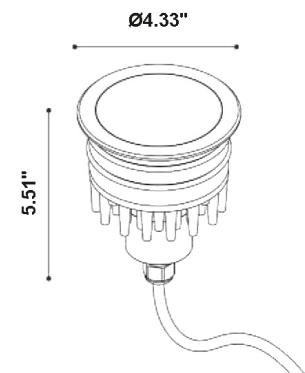
Fixture Dimensions
