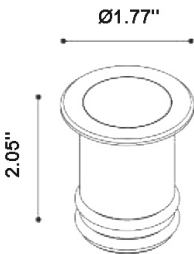
Fixture Dimensions
