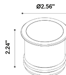
Fixture Dimensions
