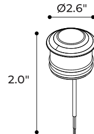
Fixture Dimensions
