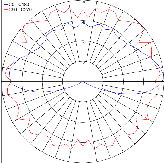
PHOTOMETRIC FILENAME : ZERO-DOME-360°-3000K.IES
