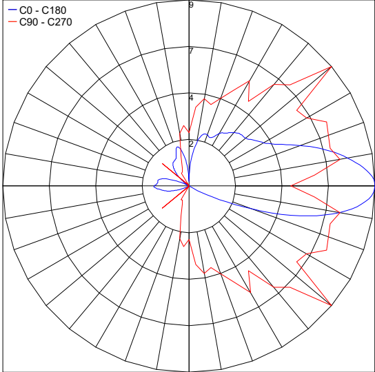
PHOTOMETRIC FILENAME : ZERO-DOME-180°-3000K.IES
