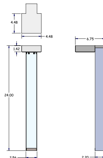
Fixture Dimensions
