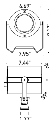
Fixture Dimensions
