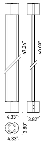
Fixture Dimensions
