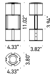
Fixture Dimensions
