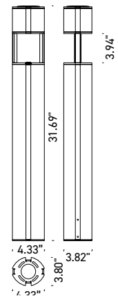
Fixture Dimensions
