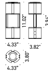
Fixture Dimensions
