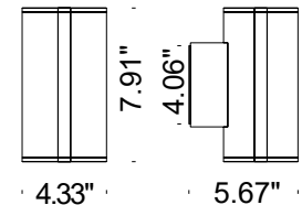
Fixture Dimensions
