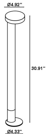
Fixture Dimensions
