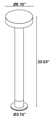
Fixture Dimensions
