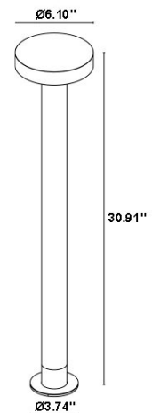
Fixture Dimensions
