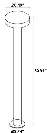
Fixture Dimensions
