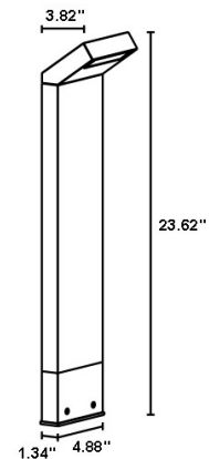
Fixture Dimensions
