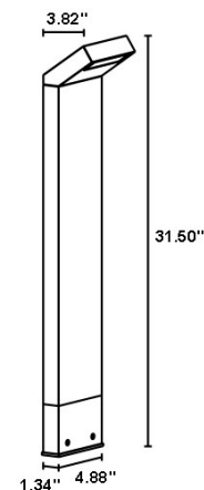
Fixture Dimensions
