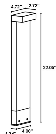
Fixture Dimensions
