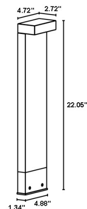
Fixture Dimensions
