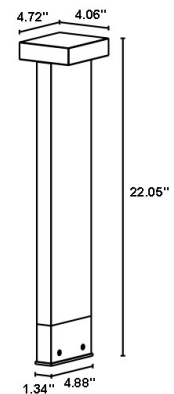
Fixture Dimensions
