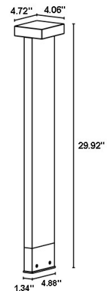
Fixture Dimensions
