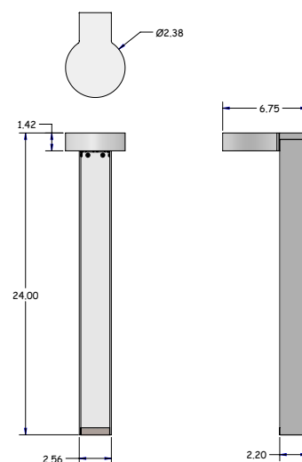
Fixture Dimensions
