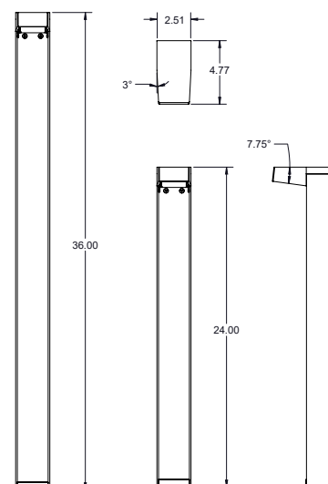
Fixture Dimensions
