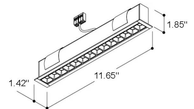
Fixture Dimensions
