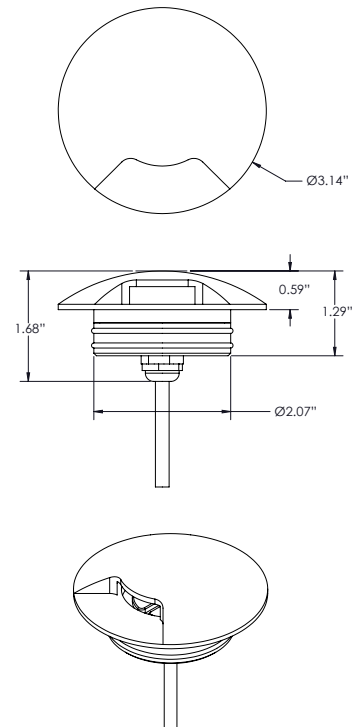
Fixture Dimensions
