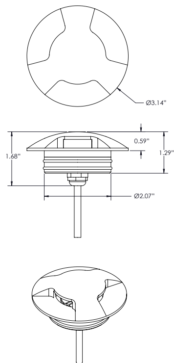
Fixture Dimensions
