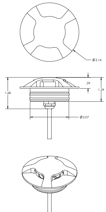
Fixture Dimensions
