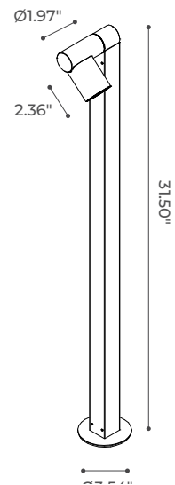
Fixture Dimensions
