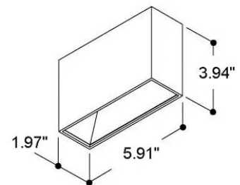
Fixture Dimensions
