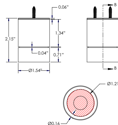
Fixture Dimensions
