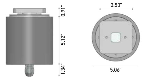
Fixture Dimensions
