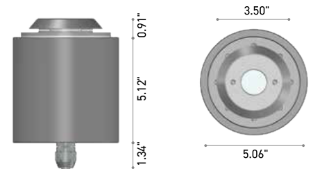
Fixture Dimensions
