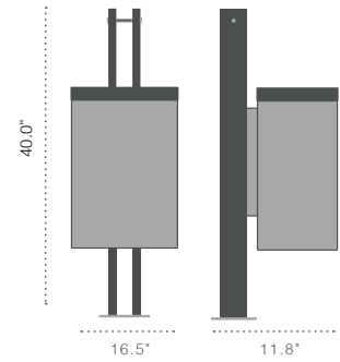
Fixture Dimensions
