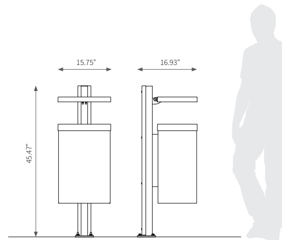
Fixture Dimensions
