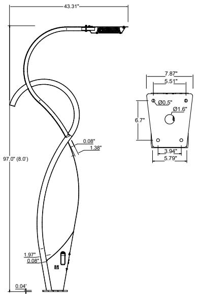
Fixture Dimensions
