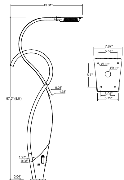
Fixture Dimensions
