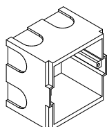
Recessed box 2.8" x 2.8" x 2.1" For Itaca 90 and 135 code 9018
