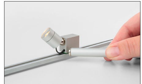
The dimming sensor is located at the cable entry in the lamp base. See more page 2.
