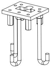
AM-00010 Mounting Base Assembly
